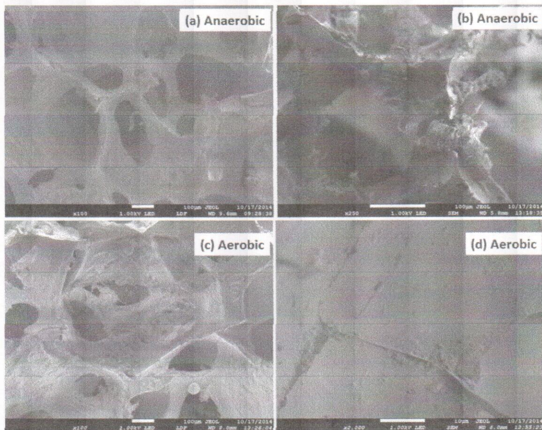
Figure 9. Microbial colonization and attached biomass to PU/(PPy-co-PANI) support in anaerobic and aerobic conditions: (a) and (c) cell aggregates in the matrix pores, (b) and (d) thin biofilms attached to the surface of support.
