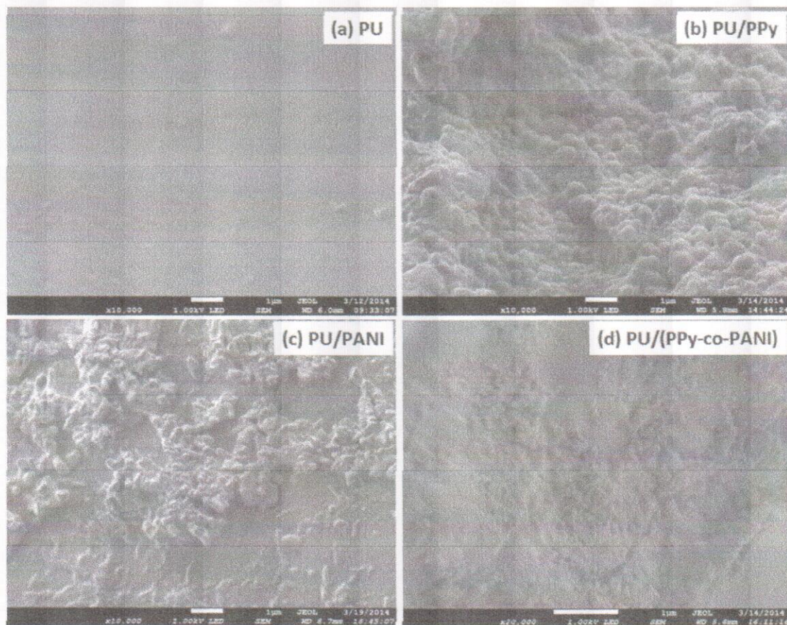
Figure 4. SEM micrographs of PU foam and different supports synthesized. (a), (b), and (c) at 10,000 \times magnification while (d) at 20,000 \times .
