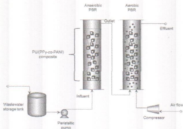
Figure 1. Flowsheet of pilot plant for municipal wastewater treatment with sequential PBR reactors.
