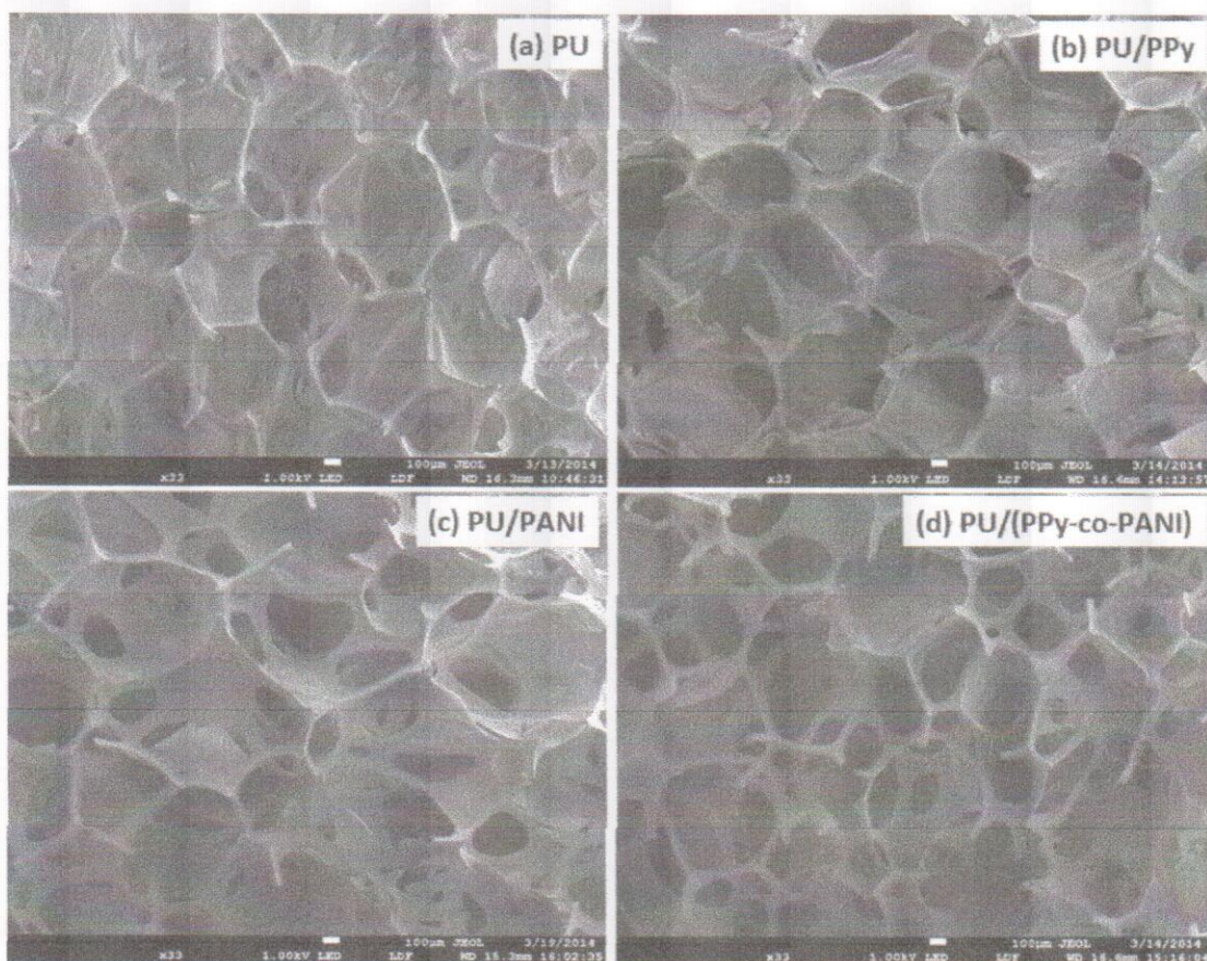
Figure 3. SEM micrographs of PU foam and different supports synthesized (33 \times magnifications).
